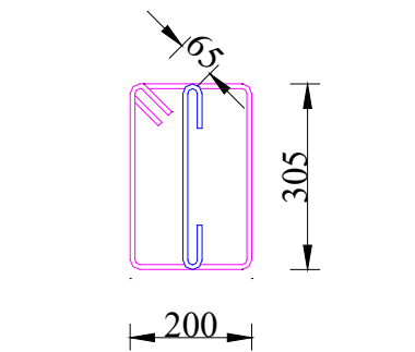
Size of Stirrups of dia 8mm
