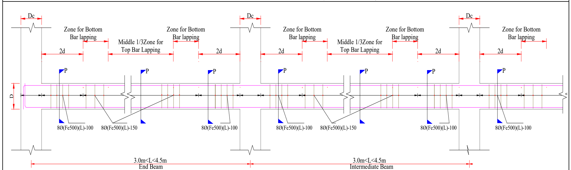
TYPICAL L-SECTION OF PLINTH BEAM (ALONG BEAM 1)
