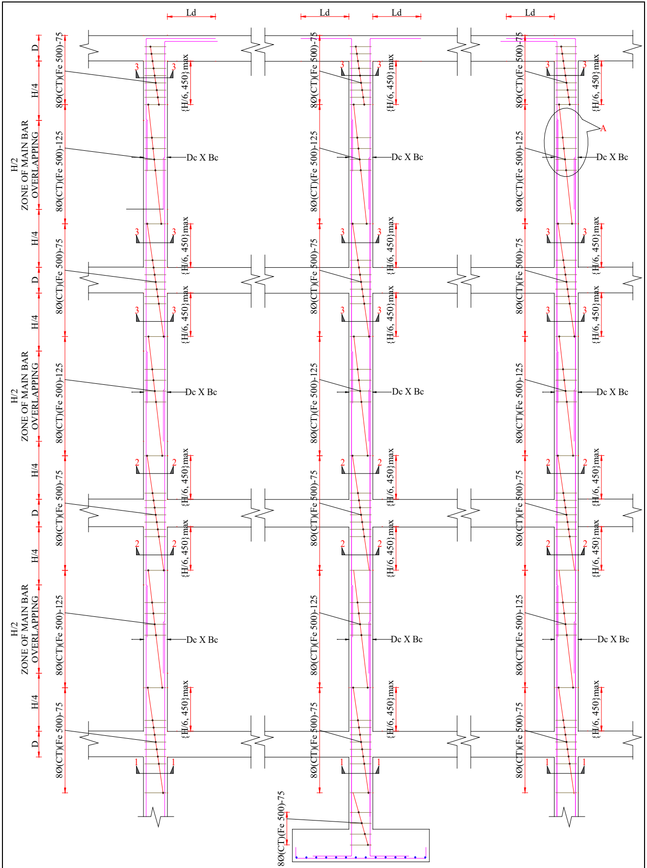
LAPPING IN COLUMN (THREE STOREY BUILDING) SECTION THROUGH INTERIOR FRAME
