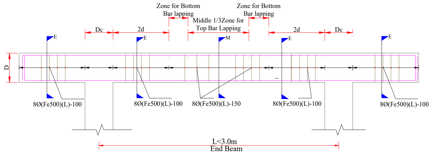
TYPICAL L-SECTION OF STAIRCOVER BEAM (ALONG BEAM 1)
