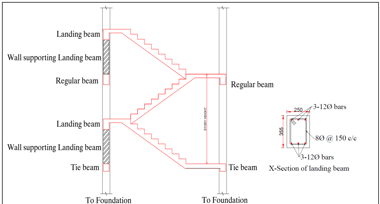
FIGURE 10-4 STAIRCASE LANDING BEAM ARRANGEMENT AND REINFORCEMENT DETAIL
