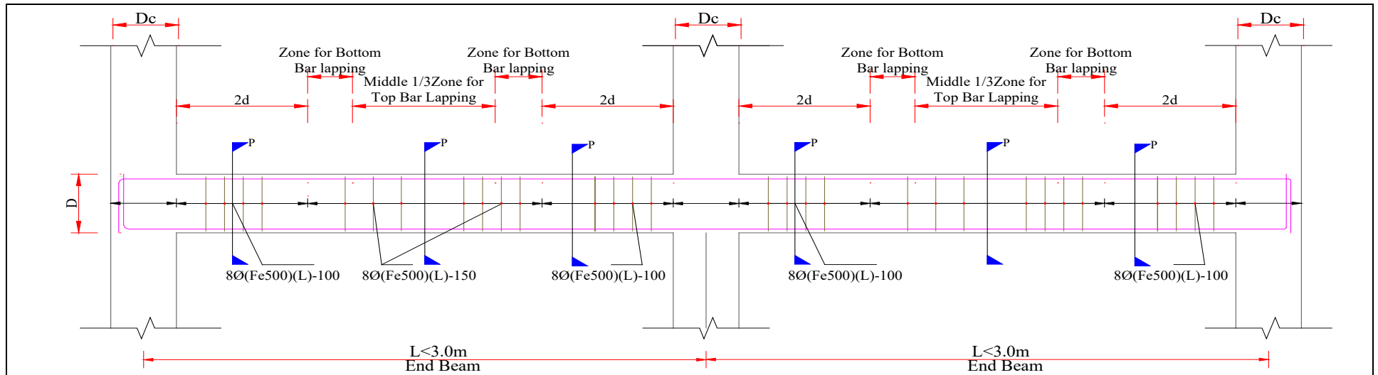
TYPICAL L-SECTION OF PLINTH BEAM (ALONG BEAM 1)
