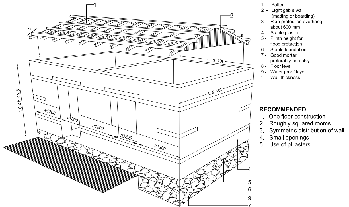
Figure 8.1: Openings for Earthen Buildings
