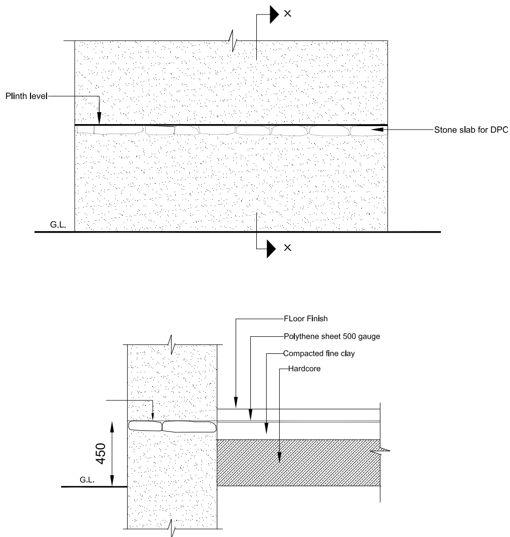
Figure 11.1: Damp-Proof Courses
