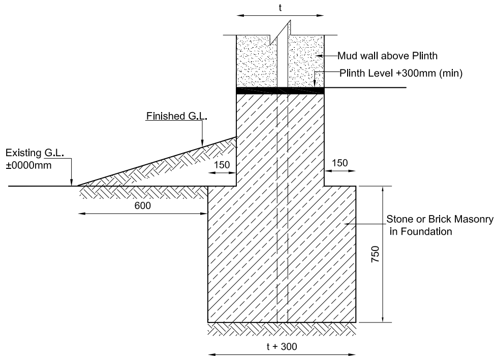
Figure 6.1: Details of Strip Foundation for an EB
