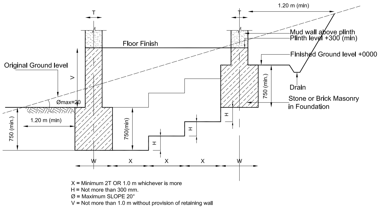
Figure6.2: Foundation on Sloping Land
