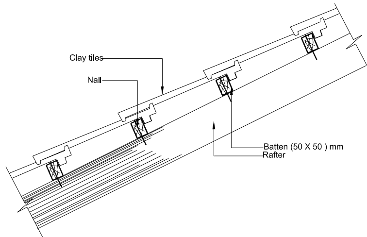
Figure 9.12: Details of Fixing Clay Tiles
