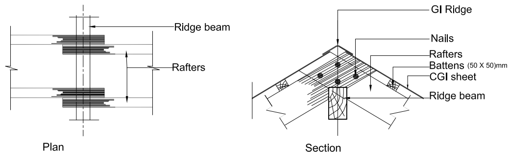
Fixing of rafters to ridge
