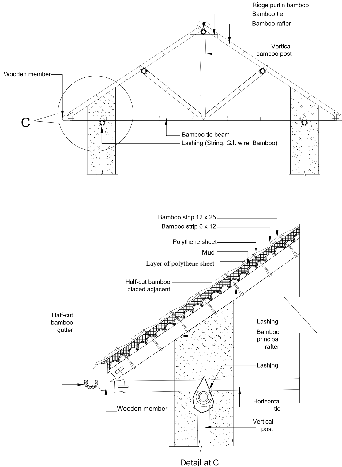
Figure 9.17: Details of Trussed Bamboo Roofing
