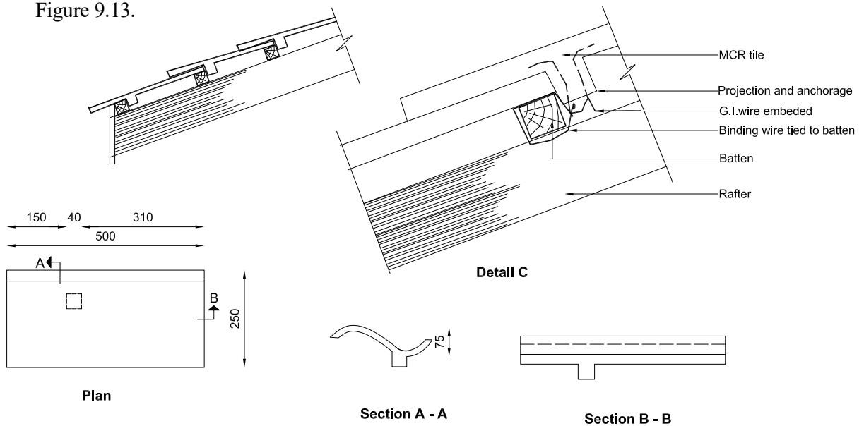
Figure 9.13: Details for Fixing MCR Tiles
