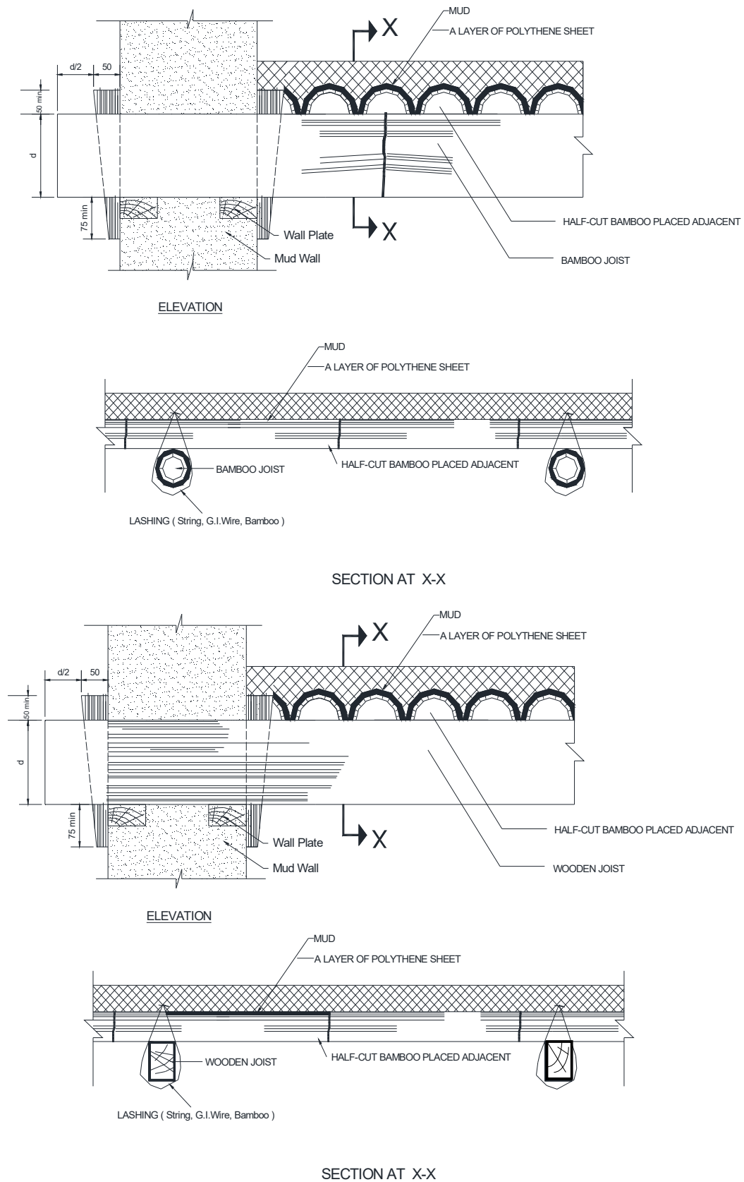
Figure 9.8: Details for Fixing Bridging Materials to Joists and Rafters
