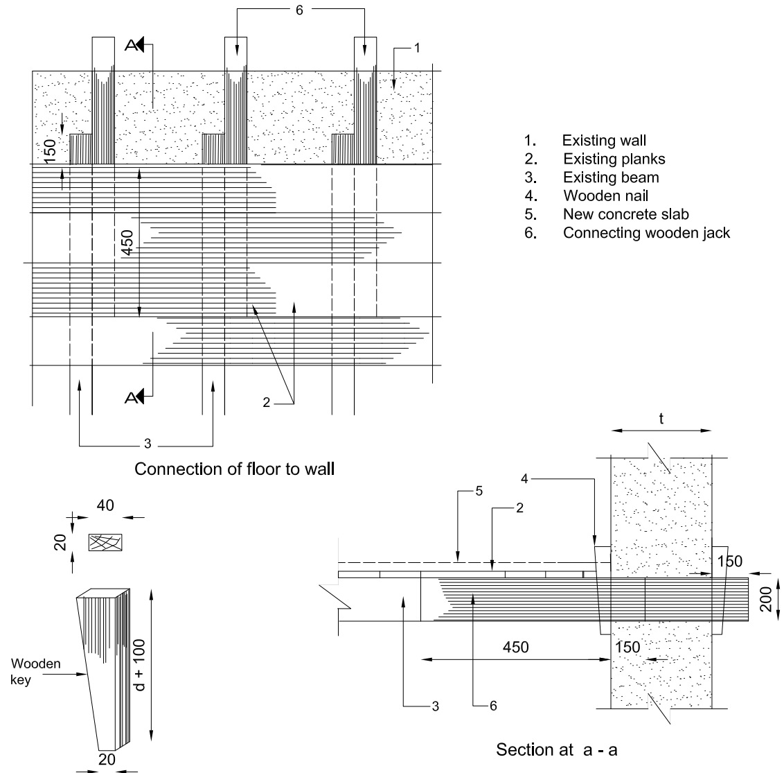
Figure 10.7: Lateral Restrainers
