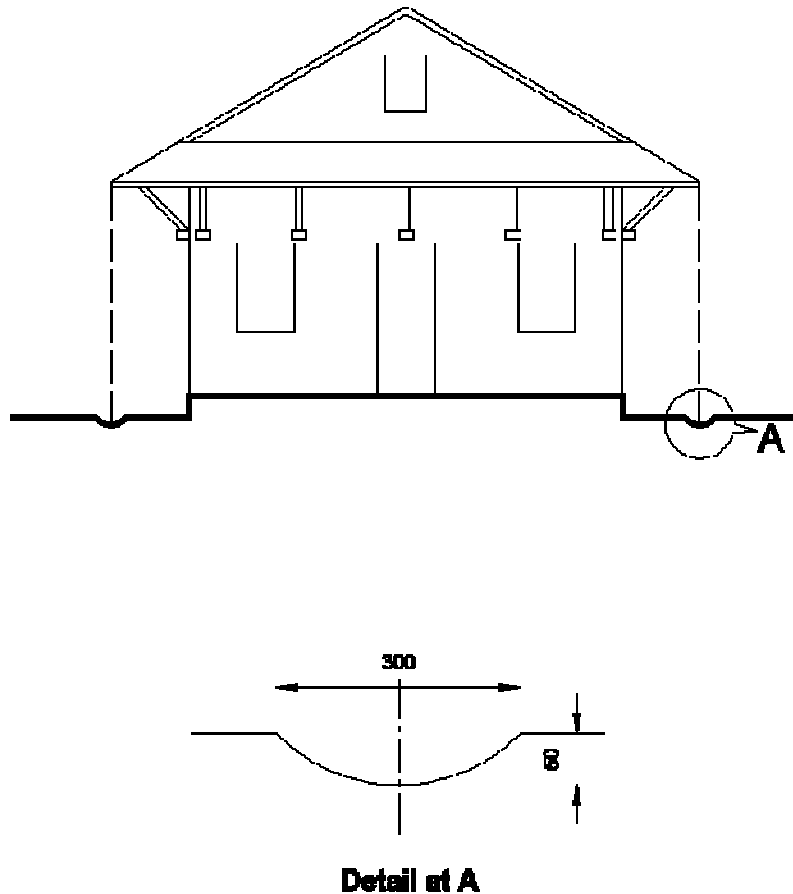
Figure 11.2: Surface Water Drainage around a Building
