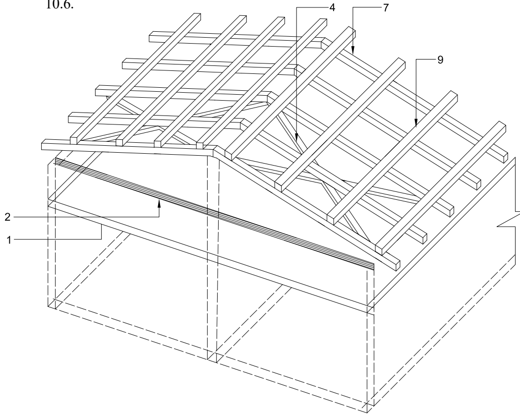
Details of roof members with bracing
