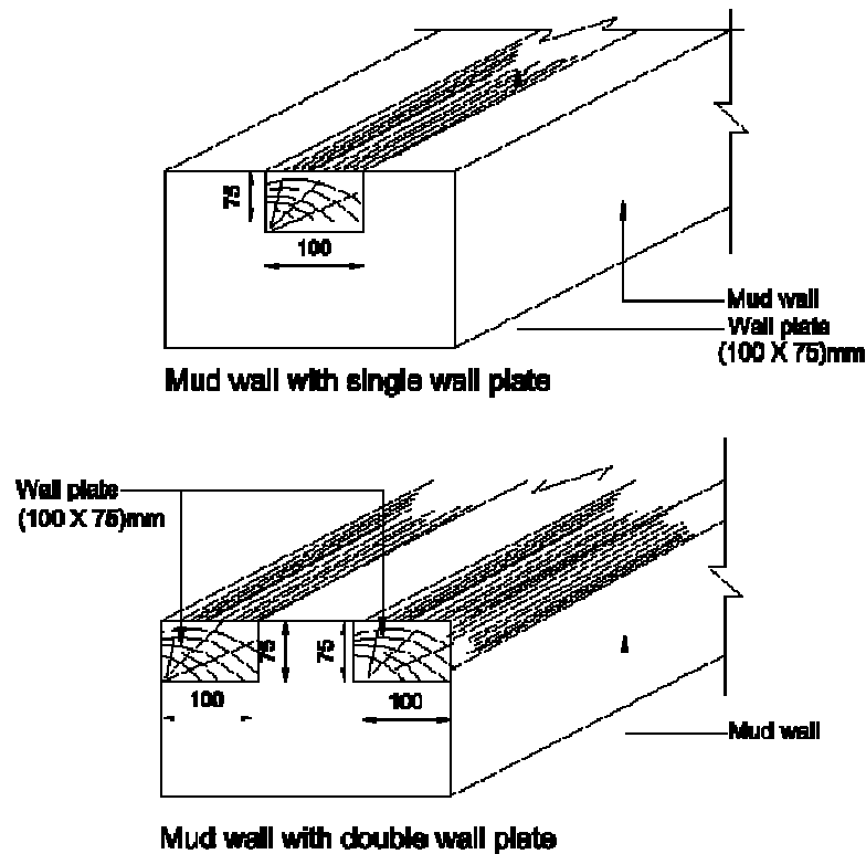
Figure 9.6: Details for Fixing Wall Plates
