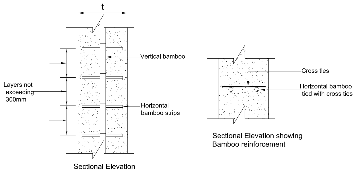
Figure 7.1: Bamboo Reinforcement Detail in Mud Wall Construction
